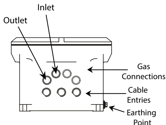
Figure 36 XTC601 Gas Connections and Cable Entries
