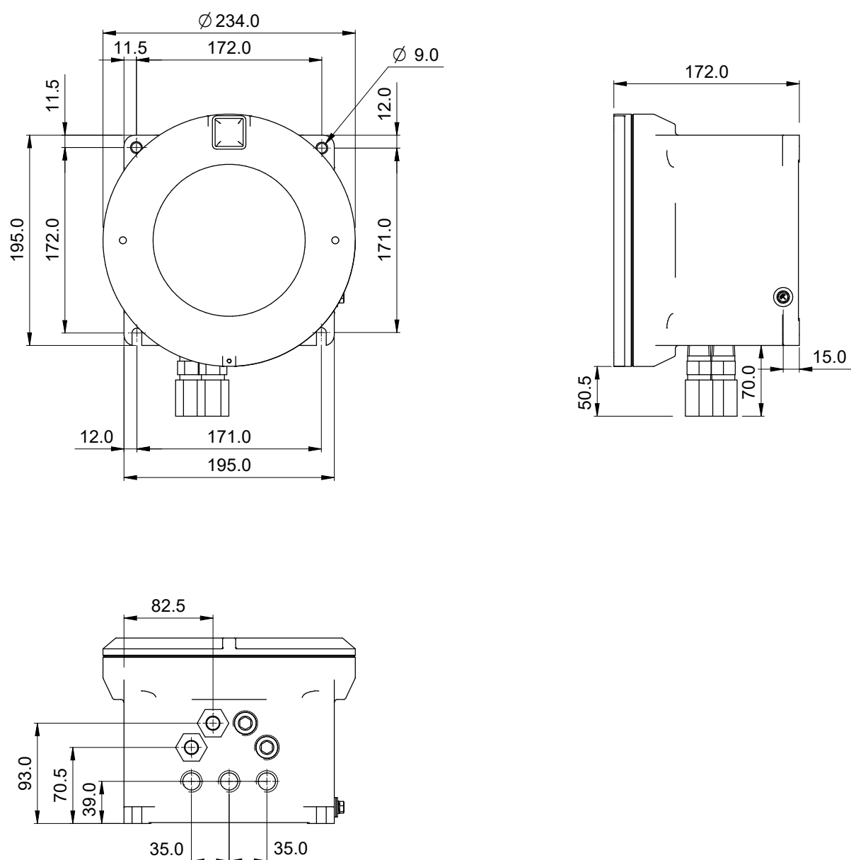
Figure 38 Dimensional Drawings
