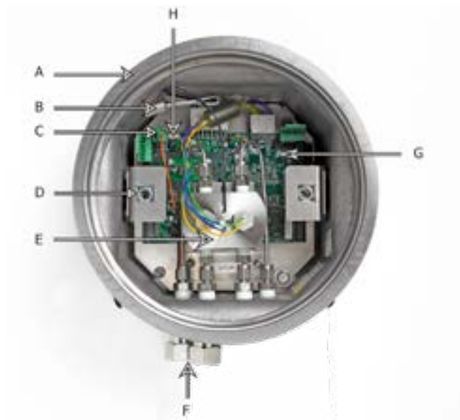
Figure 34 XTC601 Showing Major Components
