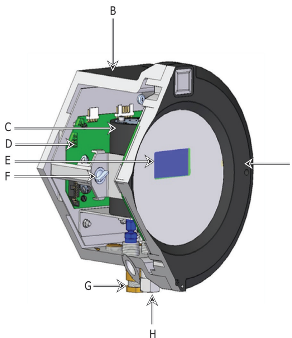
Figure 30 XTP601 Cutaway Showing Major Components
